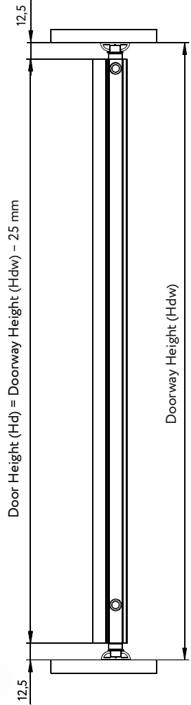
Installation with Pivot Set and Pivot Tracks
