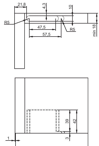
Milling of the Top Panel
